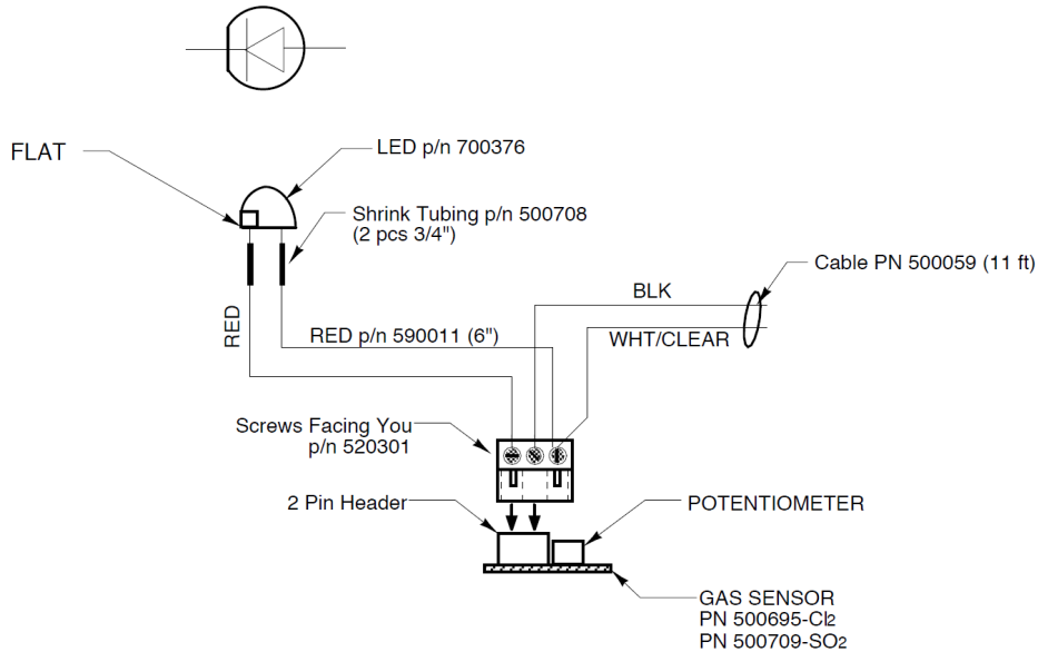
SENSOR ASSEMBLY WIRING
